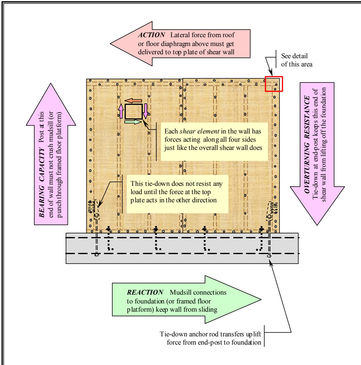
Figure 10 The four arrows in the diagram above show the forces that must act on a shear wall for it to work as intended. Shear panels nailed to the wall framing transfer forces from the top to the bottom and from one side of the wall to the other. These forces are transferred in line with each particular framing member. Because of this, the sill cannot transfer enough vertical force into the shear wall to resist overturning.
