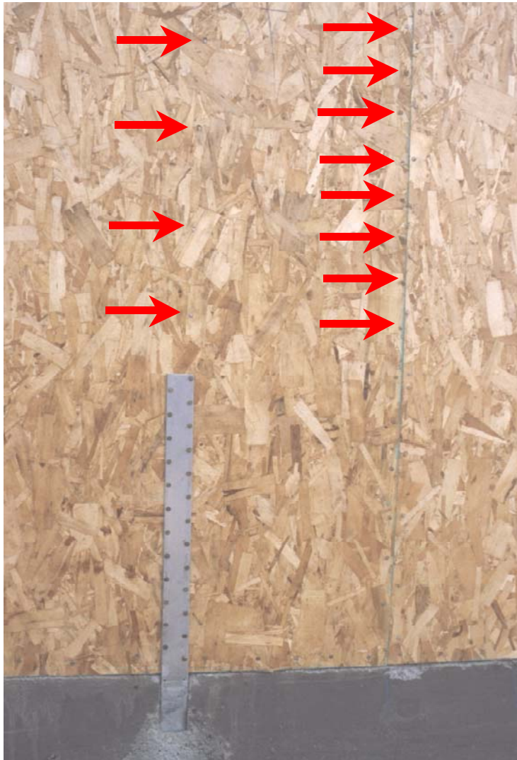
Figure 60 This strap tie-down was bent after the concrete was poured, which spalled the concrete and did not enhance the strap's capacity. The arrows highlight panel nailing. Nailing to the post behind the strap tie-down should match the panel edge nailing, but only about half the required nails are present.
